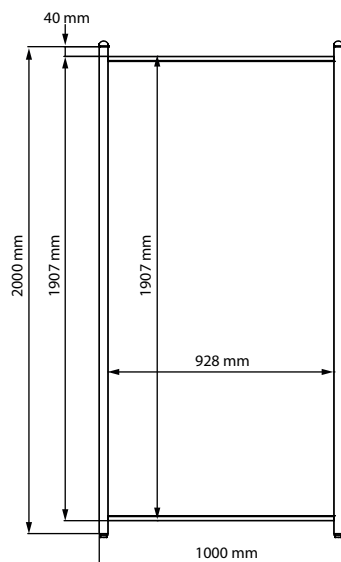
Brochure Holder
