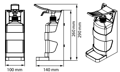
Sanitizer Dispenser Vol2 - 1 L
