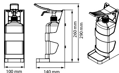
Sanitizer Dispenser Vol2 - 1 L
