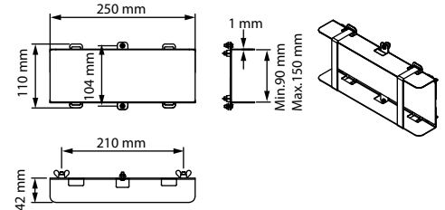
Box Bracket
