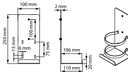
Pump Bracket
