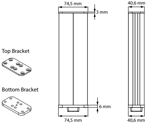
Bottom bracket Soft foot
